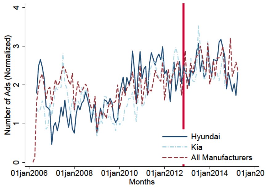
Figure C.2: The Number of Advertisements by Different Automakers
